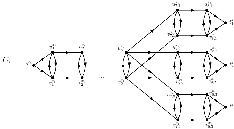
Fig. 1. The gadget G_{\phi, i} for the variable x_i .
